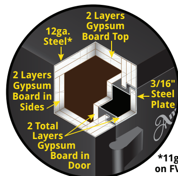
Cutaway drawing showing the FV Series interior construction
