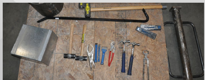
OUTSWING TEST
